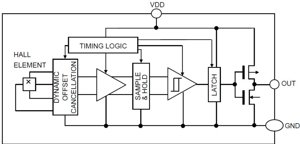
Figure 3, Block Diagram of AS1804
