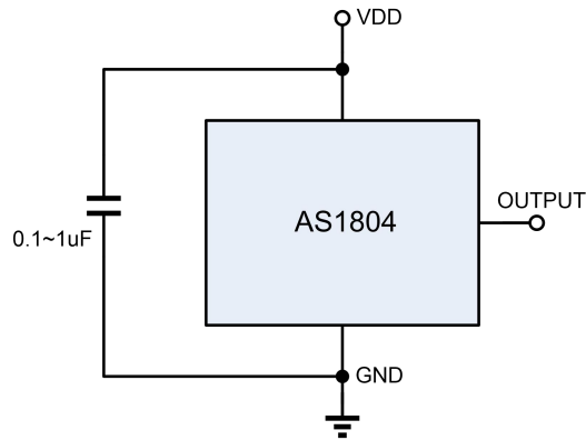
Figure 1, Typical Application Circuit of AS1804
